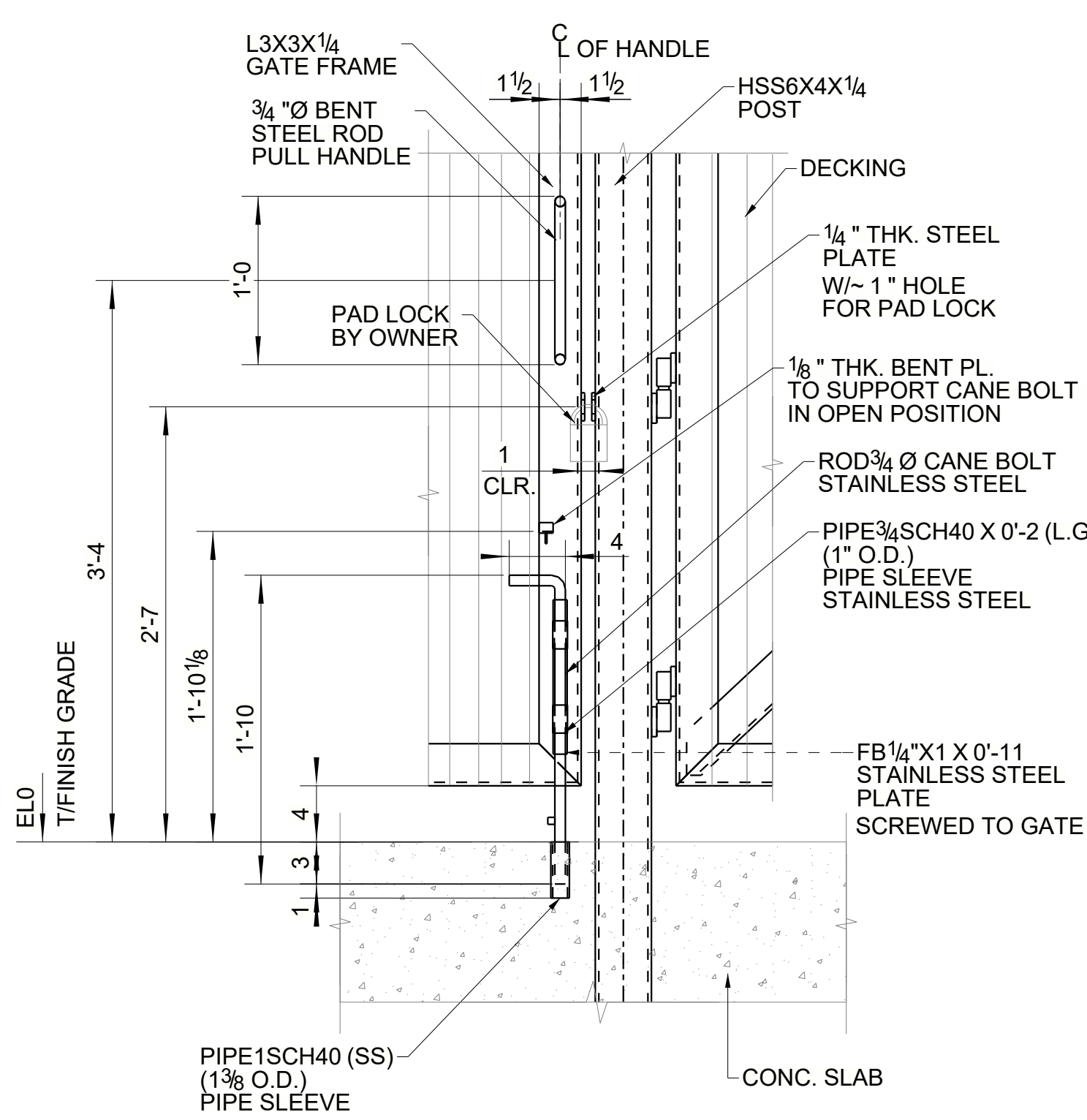
TYPICAL SINGLE GATE LOCK DETAIL
