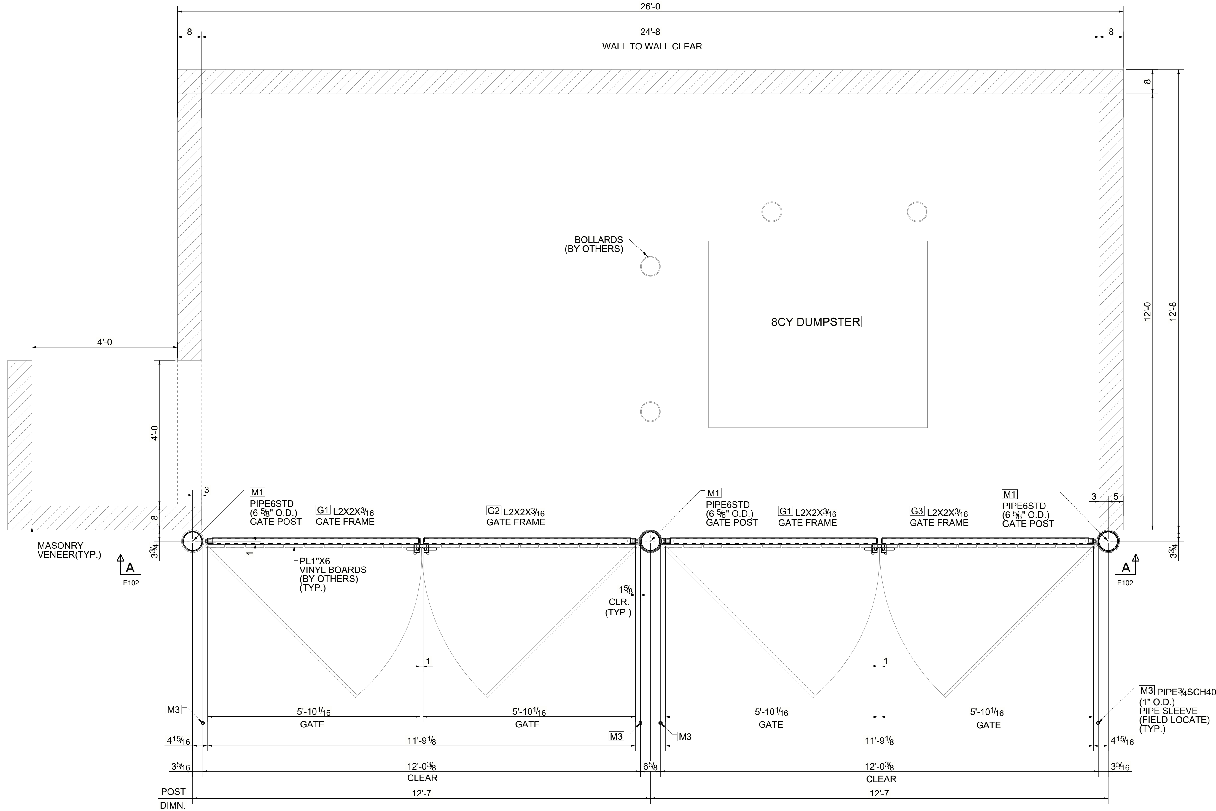
DUMPSTER GATE & BOLLARD LOCATION PLAN (REFER : DUMPSTER ENCLOSURE-11/SP7)
