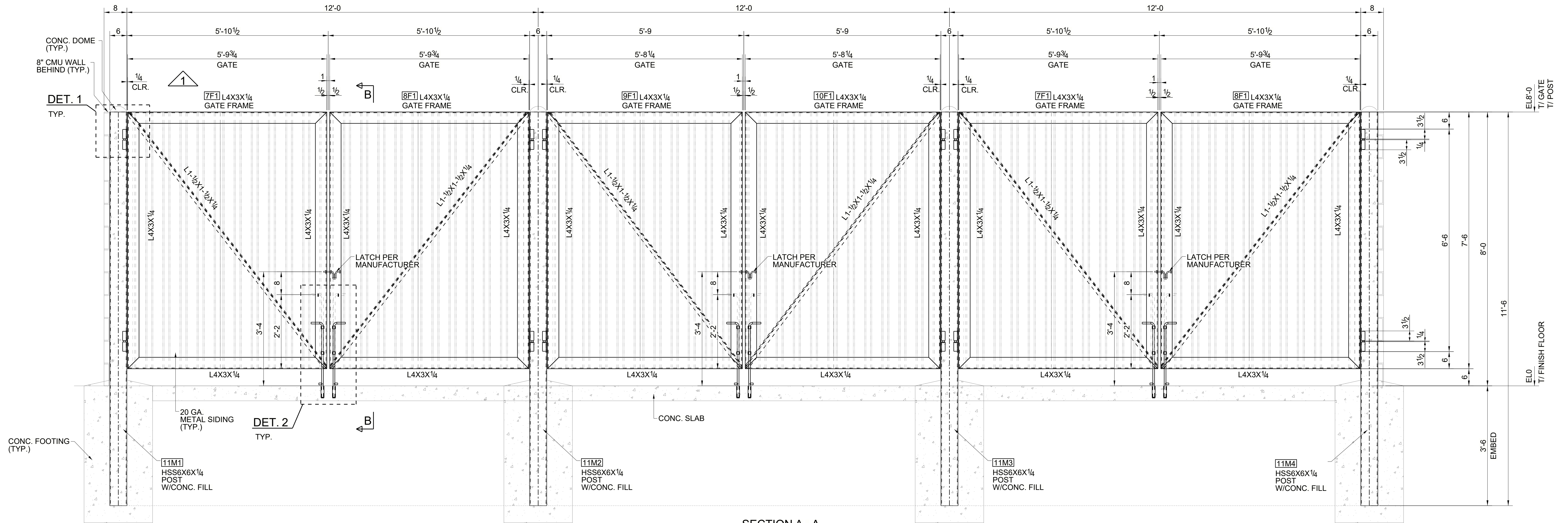
SECTION A - A E6 (REFER: TRASH ENCLOSURE - FRONT ELEVATION - 15/ SP2.1)
