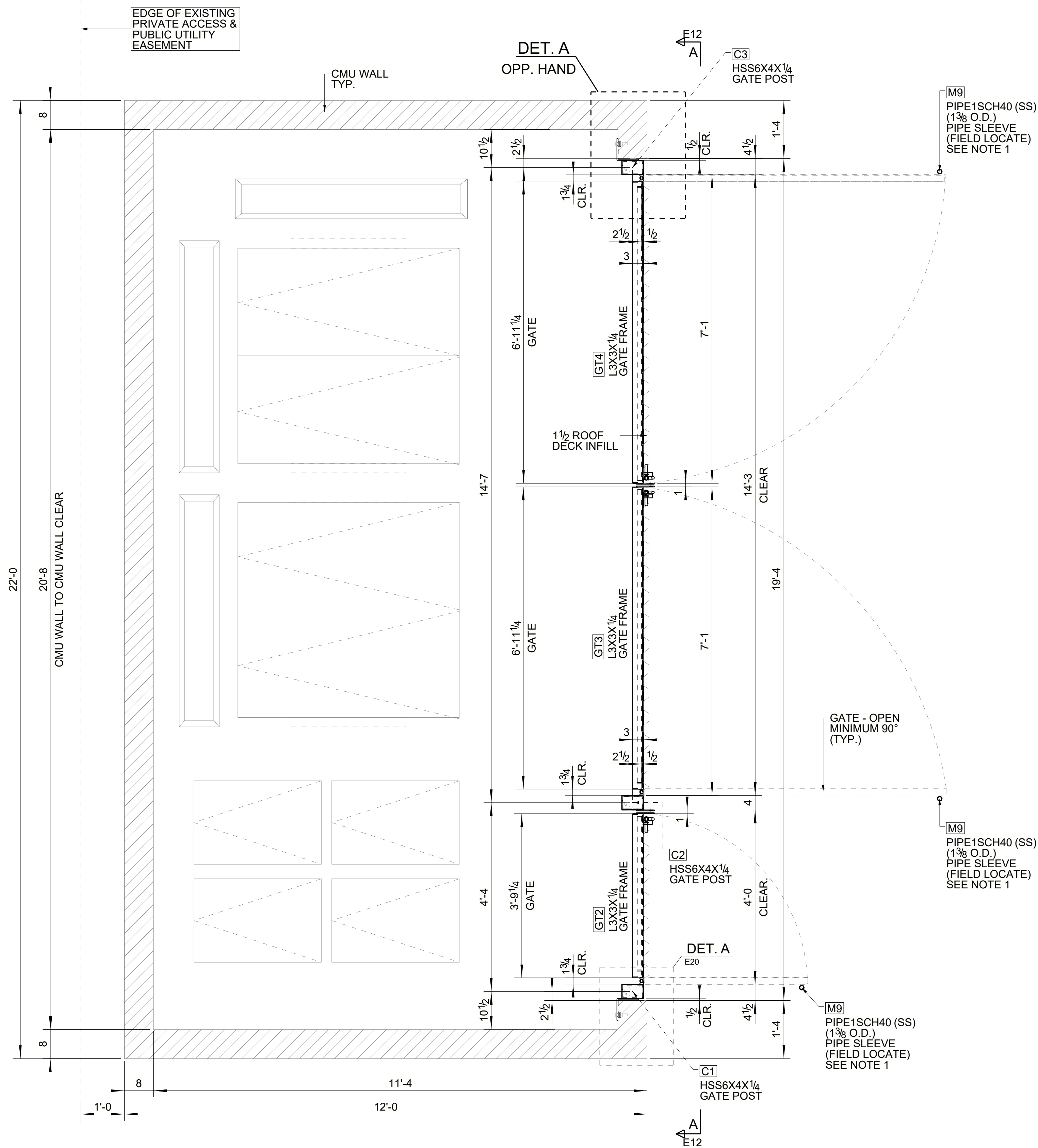
TRASH ENCLOSURE GATE LOCATION PLAN (REFER : TRASH ENCLOSURE PLAN- 6/A102 & 2/S1)
