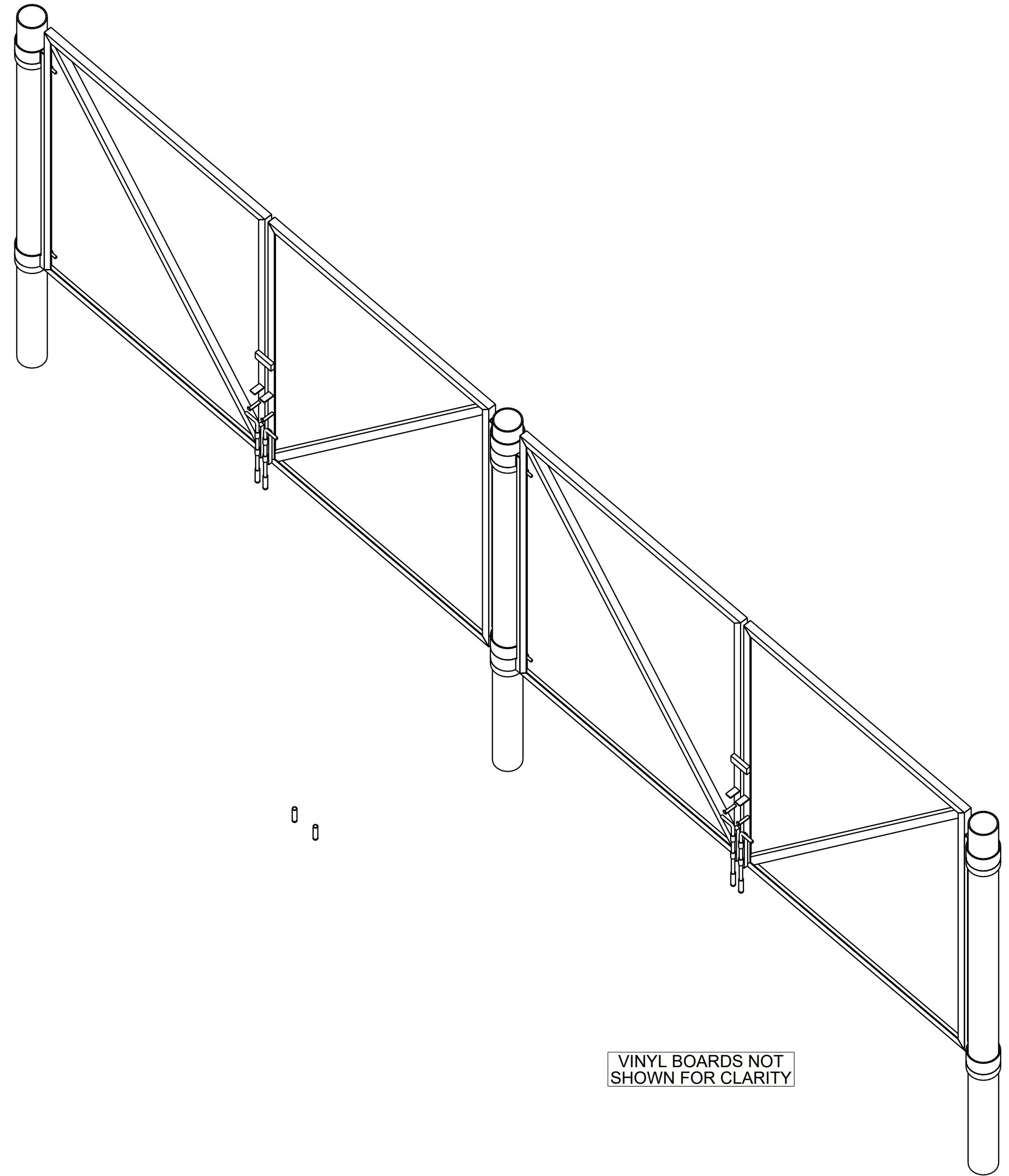
3D VIEW - DUMPSTER GATE & BOLLARD
