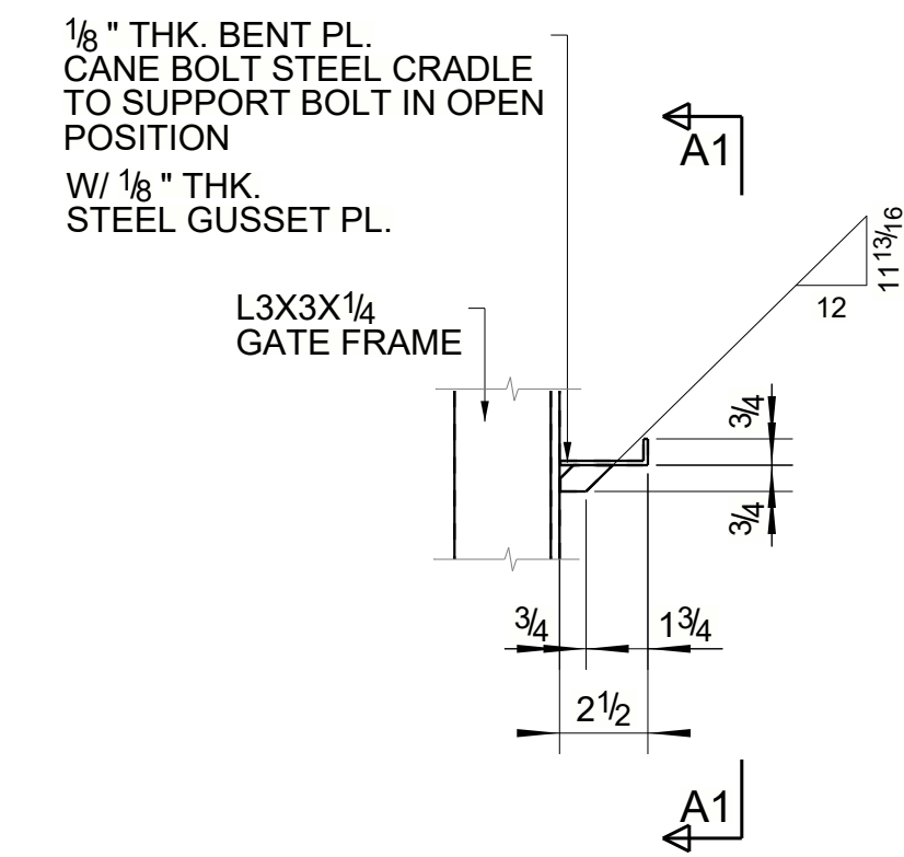
TYPICAL CANE BOLT HOLD OPEN SUPPORT TAB
