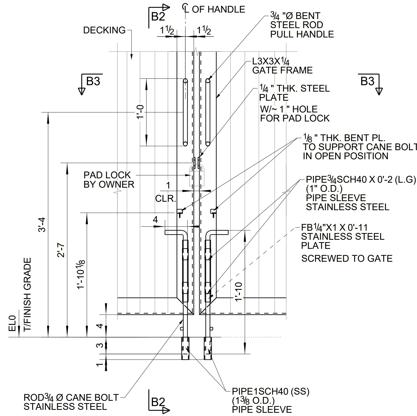
TYPICAL DOUBLE GATE LOCK DETAIL
