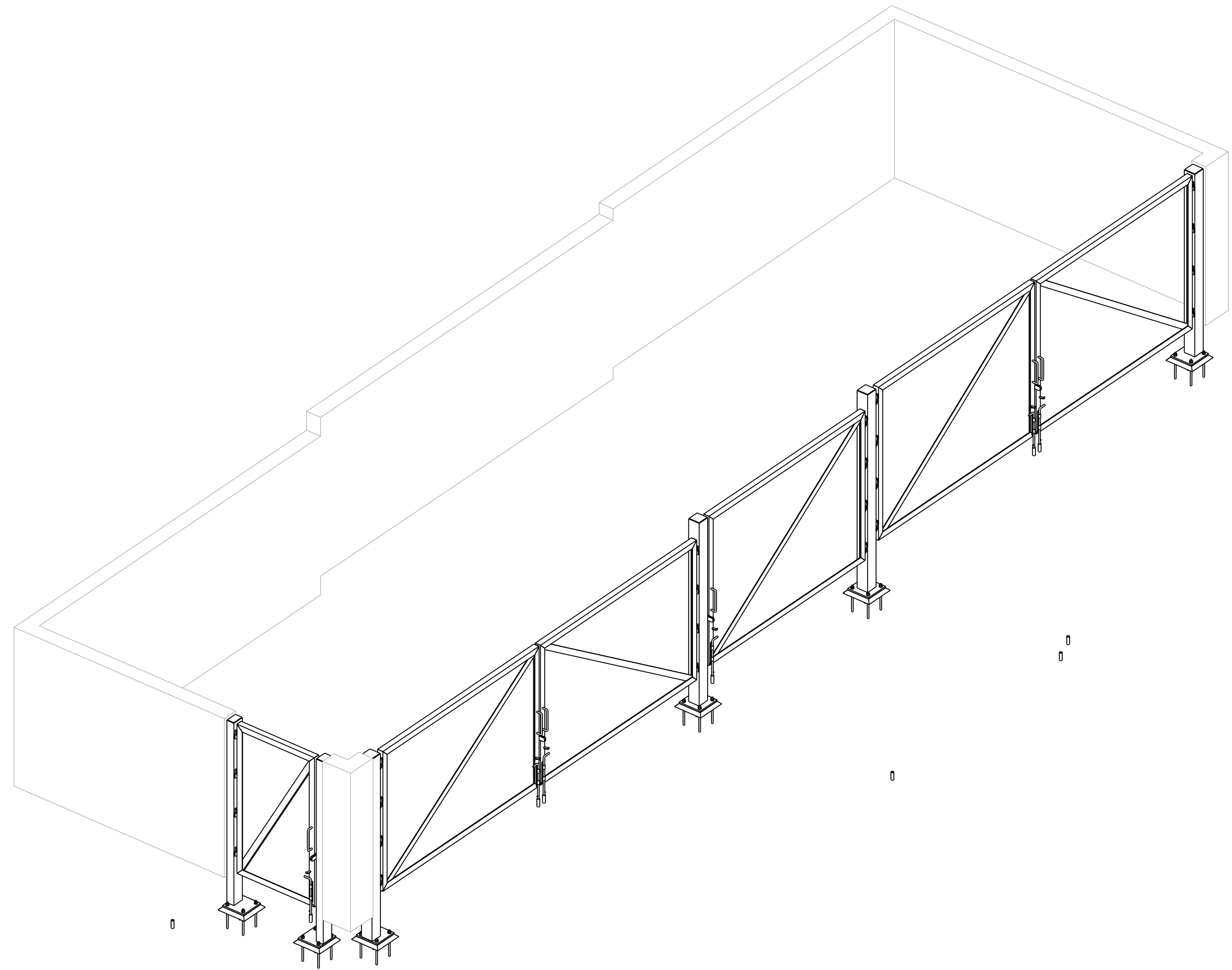
3D VIEW -LARGE TRASH ENCLOSURE GATE
