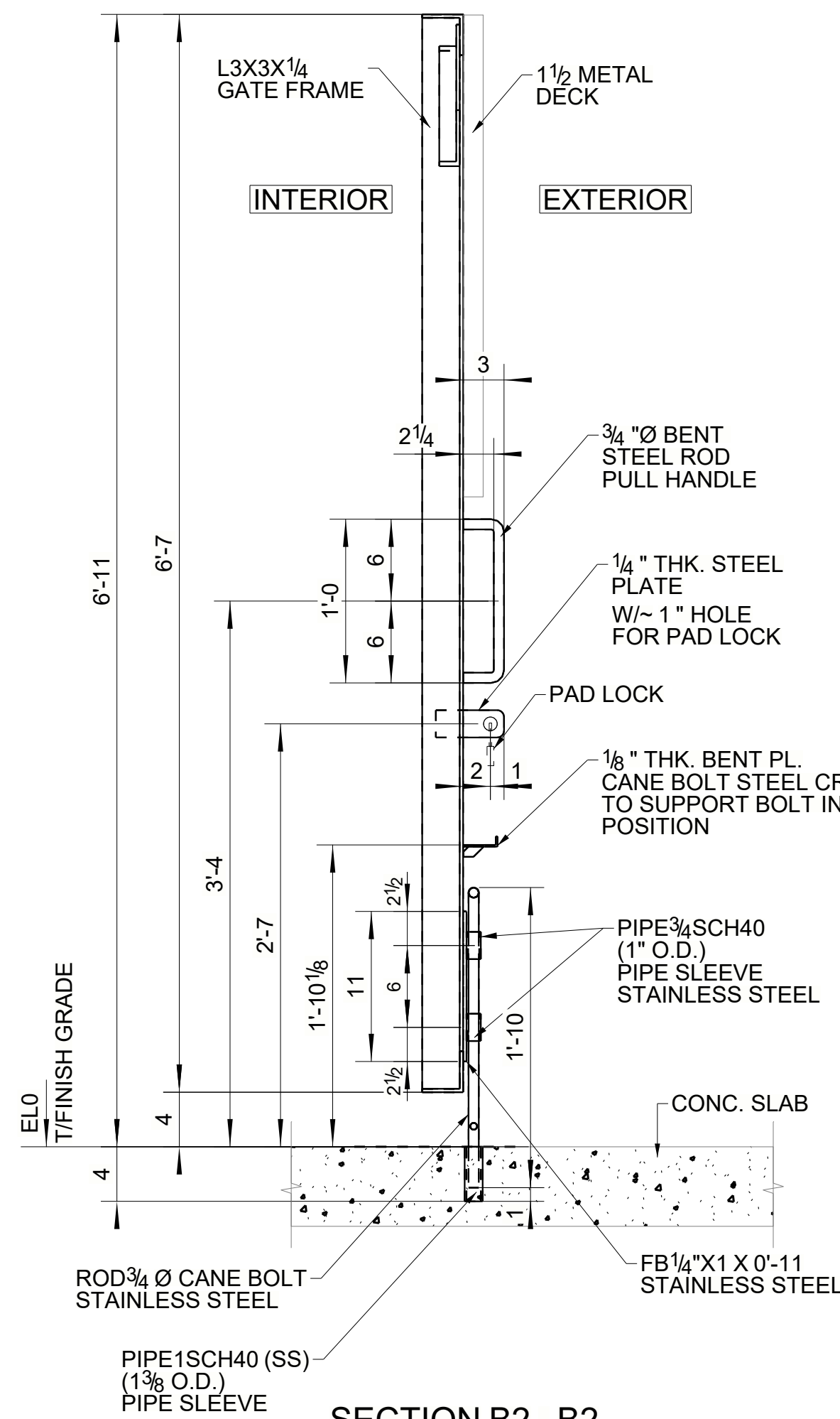
SECTION B2 - B2
