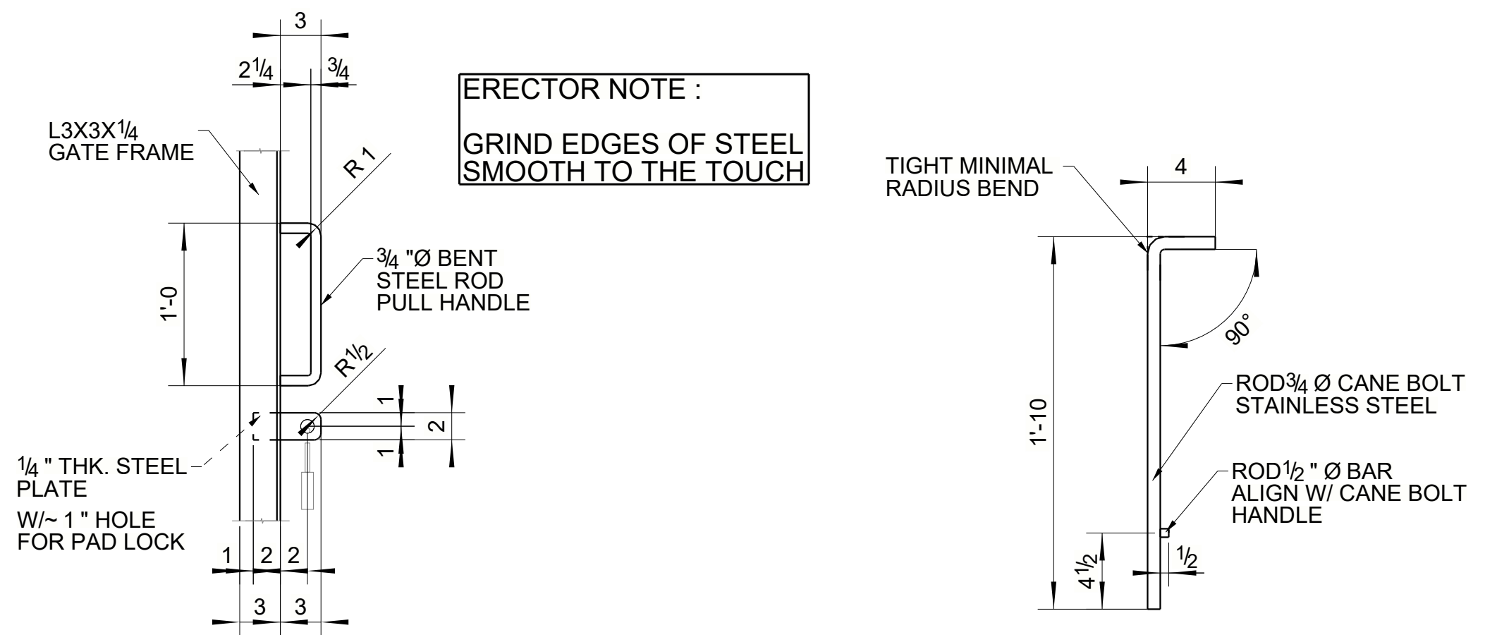
TYPICAL HANDLE AND PAD LOCK DETAIL
