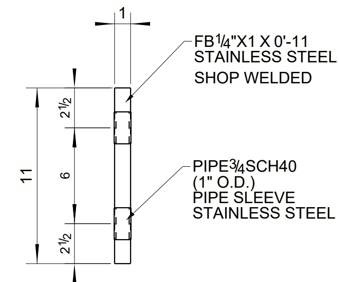
TYPICAL CANE BOLT GUIDE DETAIL
