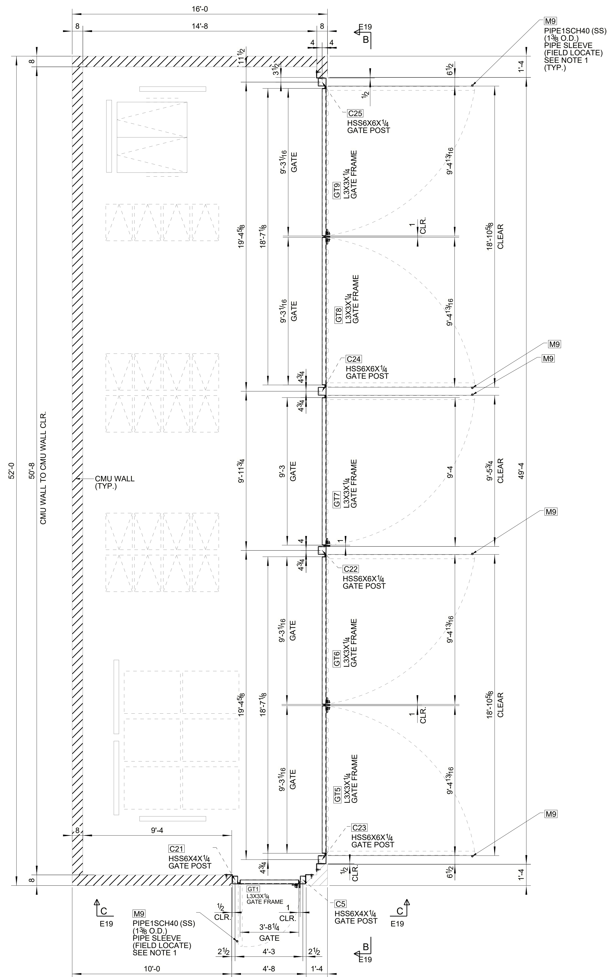
LARGE TRASH ENCLOSURE GATE LOCATION PLAN (REFER : LARGE TRASH ENCLOSURE ENLARGED PLAN- 7/A104, 8/A101.5)
